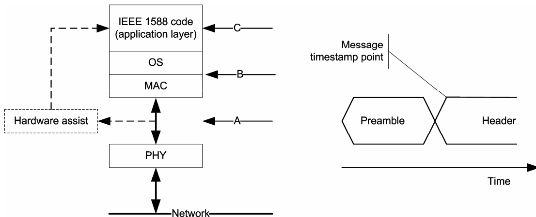
Figure 14—Timestamp generation model
