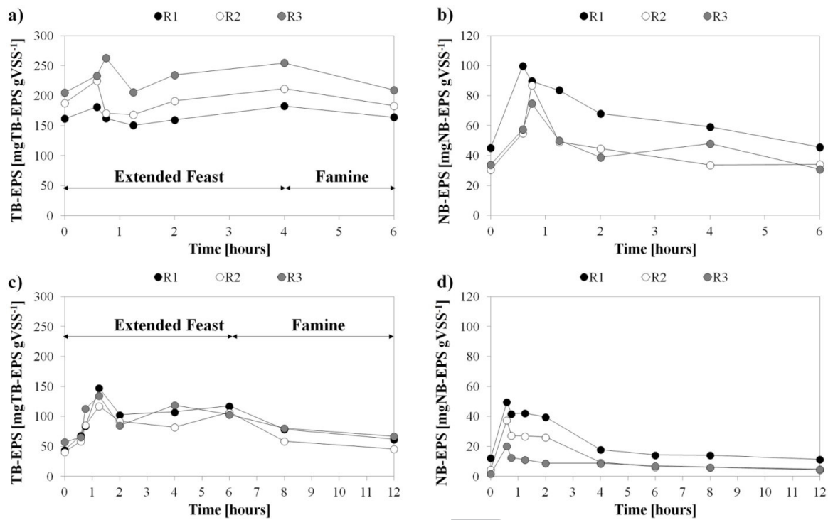
Fig.2: Specific tightly bound EPS (TB-EPS) and not bound EPS (NB-EPS) profiles during the cycle in one representative day in Period I (a, b) and Period II (c, d)
