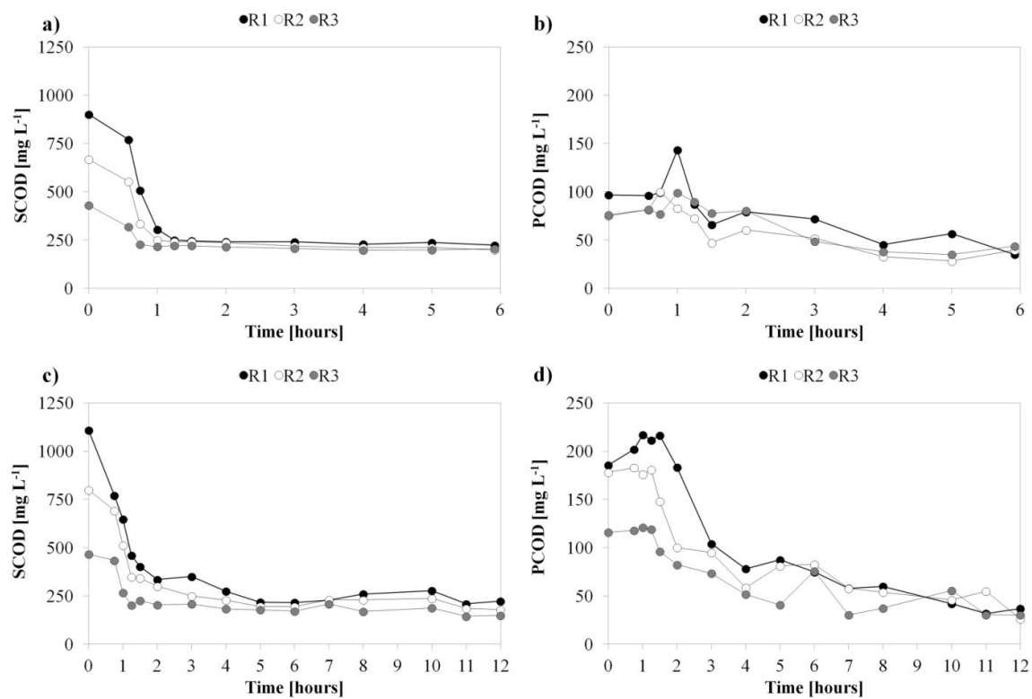
Fig.1: Soluble and particulate COD profiles during a cycle in one representative day in Period I (a, b) and Period II (c, d)
