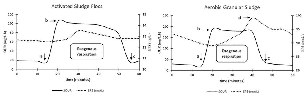
Fig. 1. Specific oxygen uptake rate (SOUR) in the oxidation of organic matter in activated sludge flocs (ASF) and aerobic granular sludge (AGS). a – addition of organic matter (120 mg/L COD – sodium acetate); b – maximum OUR; c – end of exogenous respiration; d – EPS consumption.
