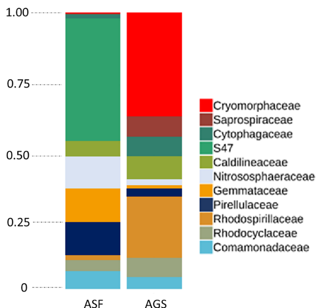
Fig. 4. Taxonomic affiliation at family level of the activated sludge flocs (ASF) and aerobic granular sludge (AGS).
