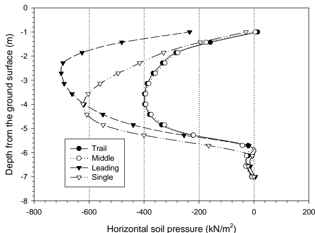
Figure 8. Lateral soil pressure in front of piles at final loading
