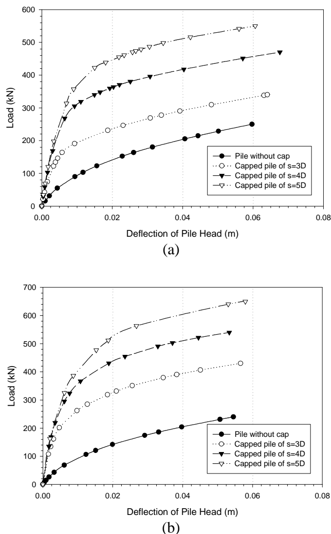
Figure 4. . Load versus deflection of single pile with diameter 0.5 m; (a). Short pile length L = 7 m, (b). Long pile length L = 10 m
