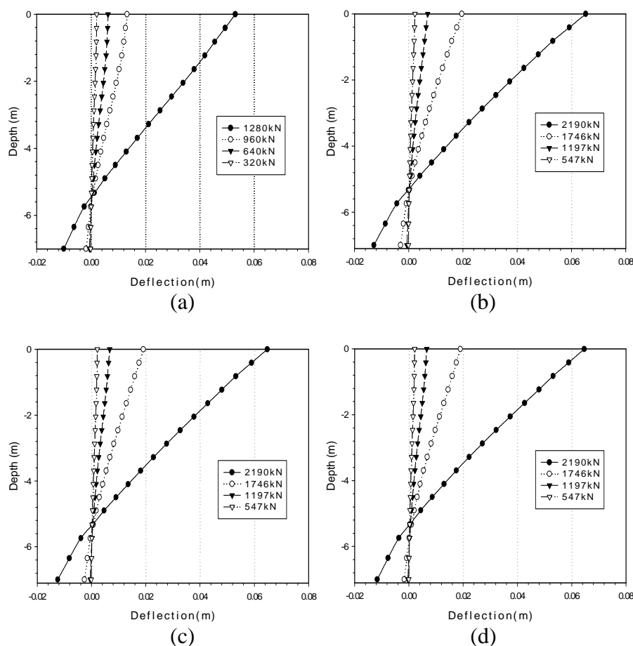
Figure 6. Deflection of pile; (a). Single pile with cap, (b). Trailing pile, (c). Middle pile, (d). Leading pile
