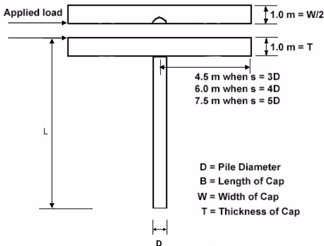
Figure 2. Layout of single pile with cap
