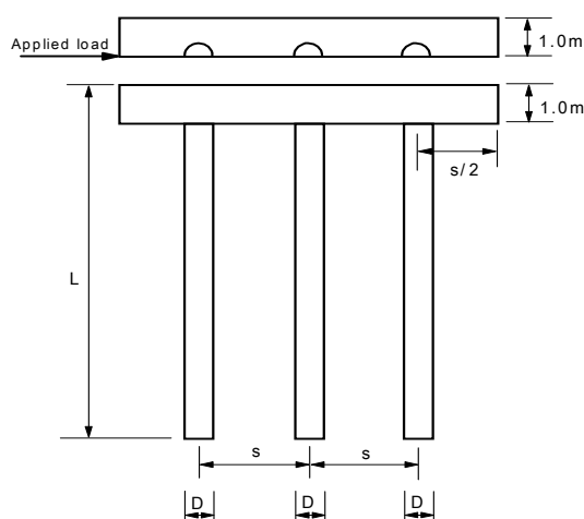
Figure 5. Cross section pile group
