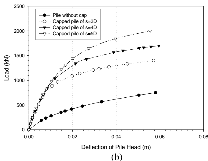
Figure 3. Load versus deflection of single pile with diameter 1.0 m; (a): Short pile length L = 7 m, (b): Long pile length L = 10 m
