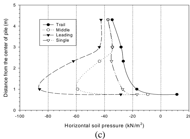
Figure 9. Lateral soil pressure on transversal plane; (a). At depth 0.43 m, (b). At depth 1.29 m, (c). At depth 2.15 m
