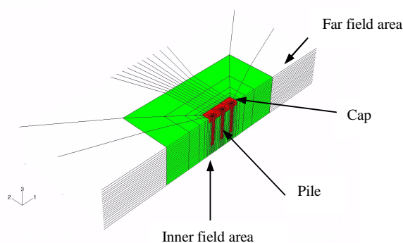
Figure 1. Finite element model of pile group
