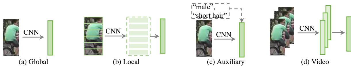
Fig. 2: Four different feature learning strategies. a) Global Feature, learning a global representation for each person image in § 2.1.1; b) Local Feature, learning part-aggregated local features in § 2.1.2; c) Auxiliary Feature, learning the feature representation using auxiliary information, e.g., attributes [71], [72] in § 2.1.3 and d) Video Feature, learning the video representation using multiple image frames and temporal information [73], [74] in § 2.1.4.
