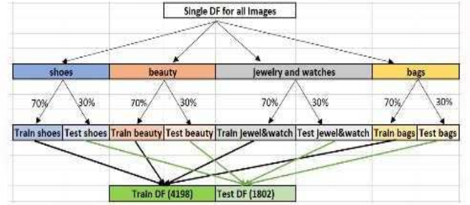
Fig. 5. The dataset needs to be split into 2 sections, train and test data sets where the train data set is used to train the model and the test dataset is used to test the validity accuracy for the given. Model. The split ratio is respectively 70:30.
