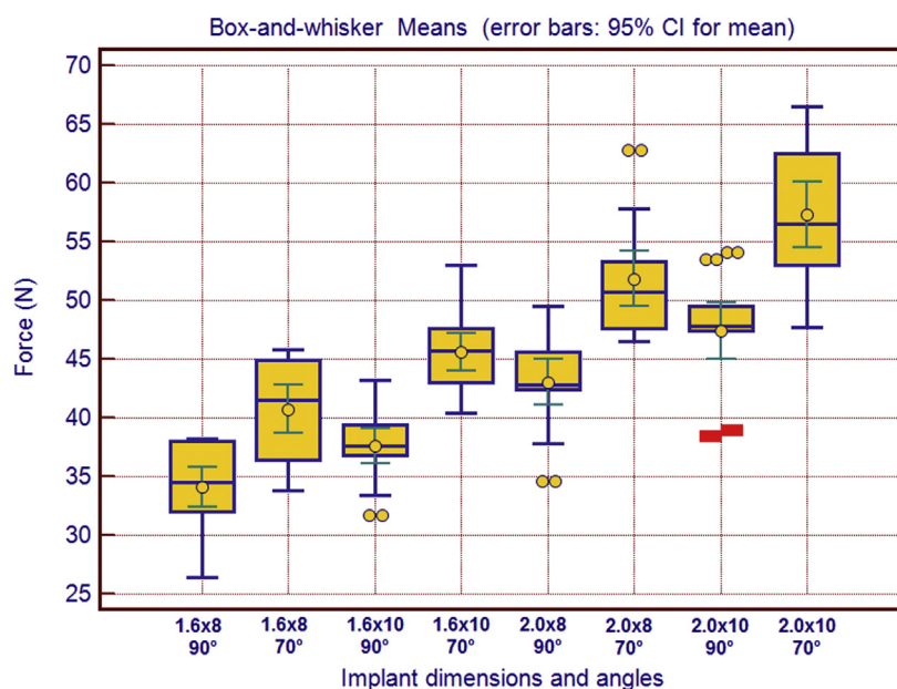
Fig 3. Box-and-whisker diagram showing the anchorage force values (N) of orthodontic mini-implants with different dimensions and insertion angles.
