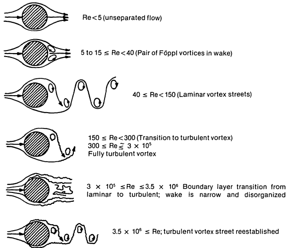
Fig. 16.4.1. Flow regimes across isolated circular cylinders [Ref. 16.4.1].
