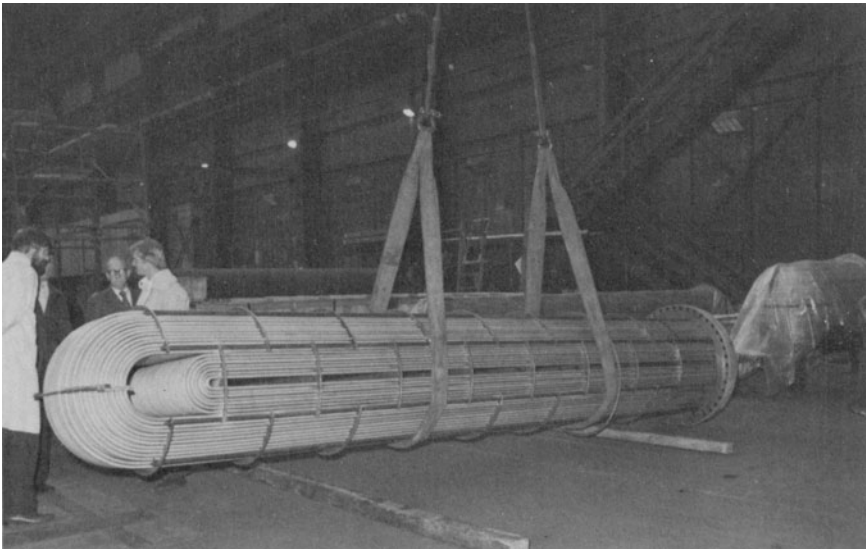
Photograph 22.e. Lifting a U-bundle using straps.
