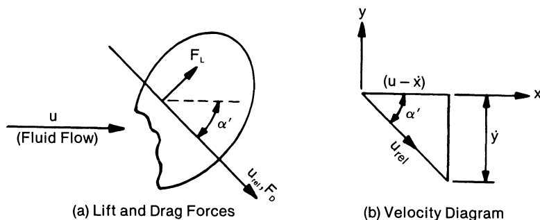
Fig. 16.4.3. Fluid flow past a bluff body.
