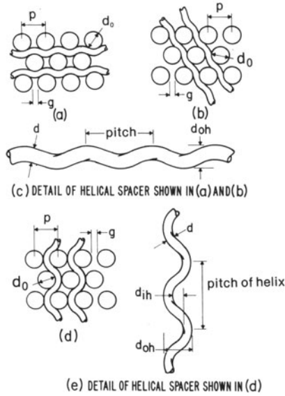
Fig. 16.12.6. Helical spacer positioned in a triangular pitch tube array in three possible directions.
