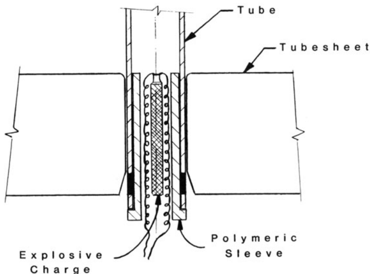
Fig. 7.5.1. Impact welding.
