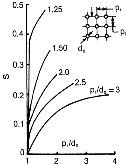
Fig. 16.7.9. Strouhal number for in-line banks of plain tubes.
