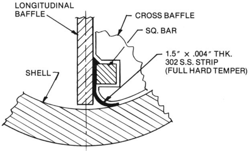
Fig. 1.4.3. Typical longitudinal baffle edge seal detail.
