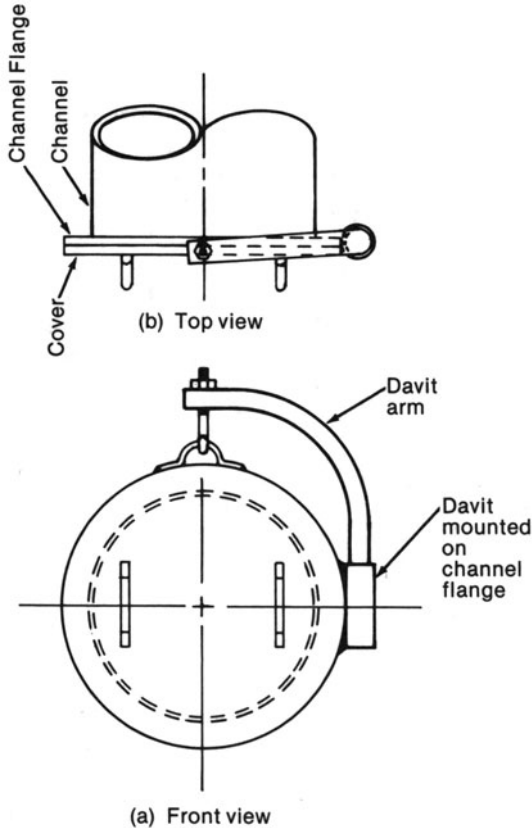
Fig. 12.1.2. Flat cover equipped with a davit arm.
