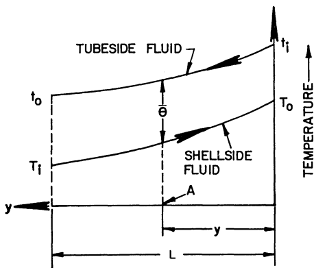
Fig. 9.5.1. Fluid temperature profiles.
