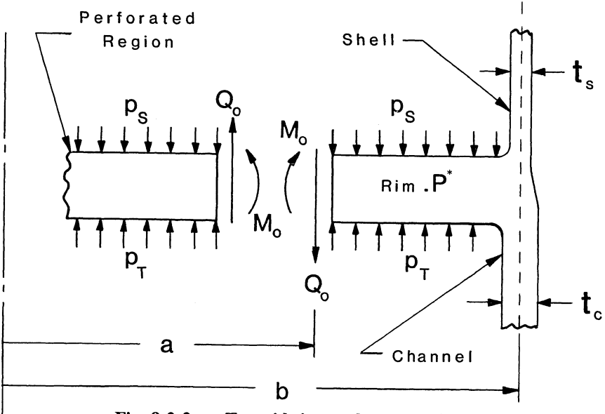
Fig. 8.2.2a. Two side integral construction.
