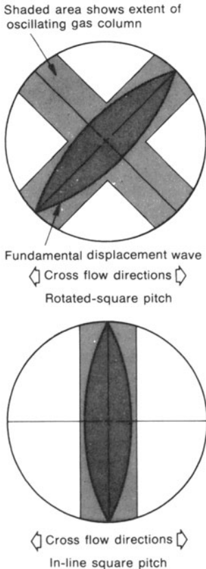
Fig. 16.7.11. Position of diametral standing wave.
