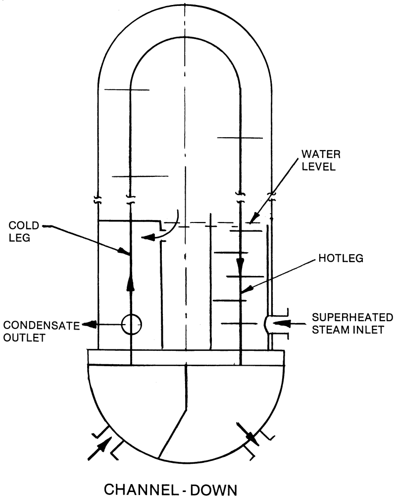
Fig. 1.10.1. Channel – down, three zone vertical feedwater heater.
