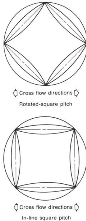
Fig. 16.7.12. Position of inscribed square standing wave.
