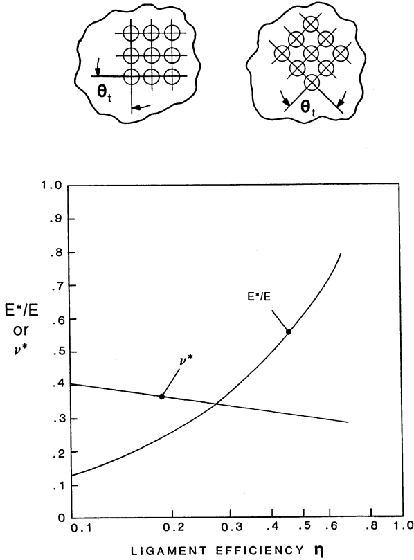
Fig. 8.1.2. Effective elastic constants-square pattern.
