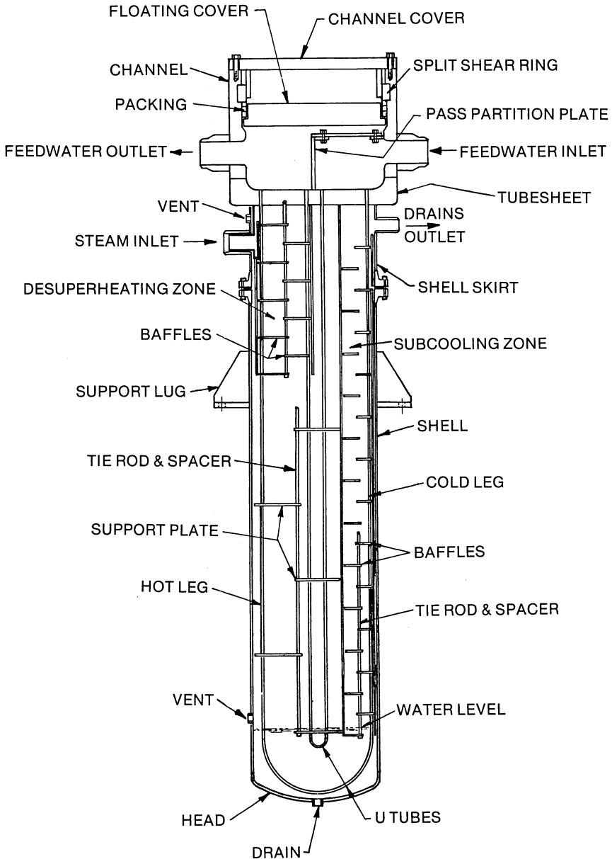
Fig. 1.10.2. Vertical feedwater heater three-zone two-pass channel up.
