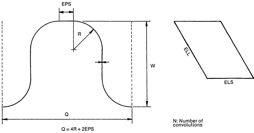
Fig. 15.B.1. Convolution geometry (code EJMAREC).
