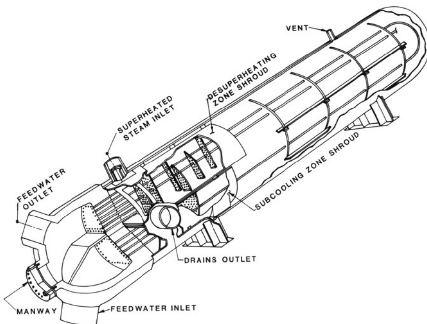
Fig. 1.2.4. Cutaway view of a three-zone horizontal feedwater heater.
