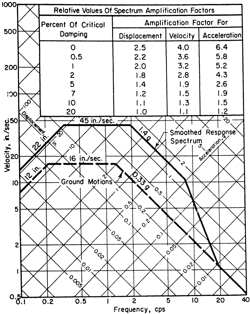
Fig. 21.2.5. Smoothed tripartite logarithmic response spectrum for 0.33 g earthquake, 2 percent critical damping.
