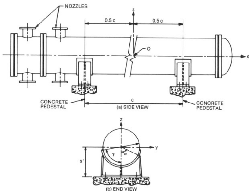
Fig. 19.1.1. A saddle supported heat exchanger.
