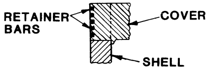
(c) CROSS-SECTIONAL VIEW
