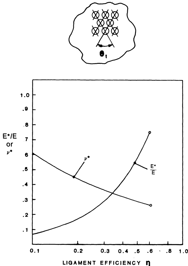
Fig. 8.1.1. Effective elastic constants – triangular pattern.
