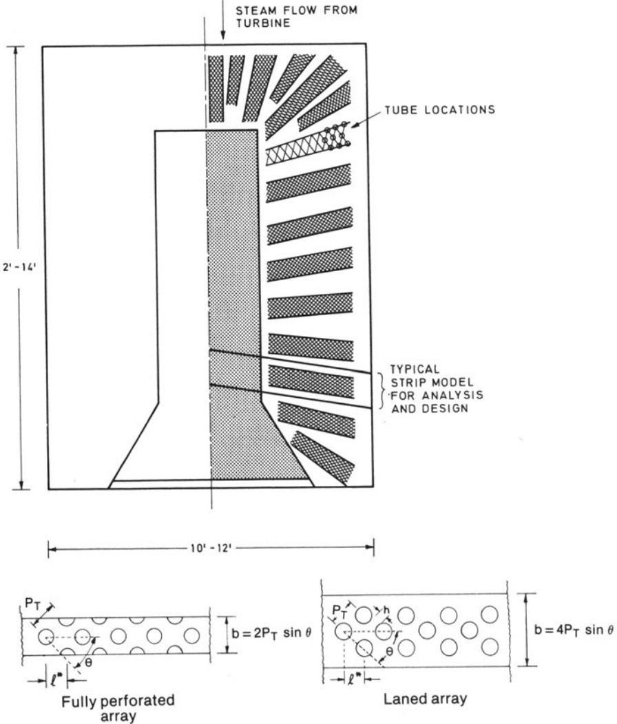
Fig. 11.2.3. Tubeshheet layout showing beam strips.
