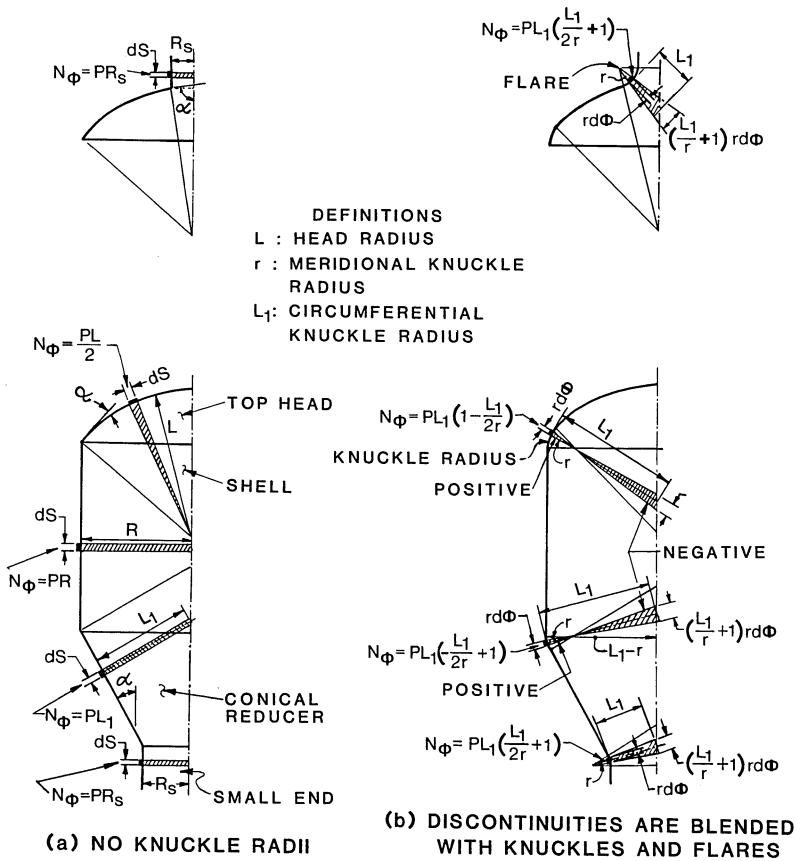
Fig. 13.5.3. Illustration of unsupported area principle.
