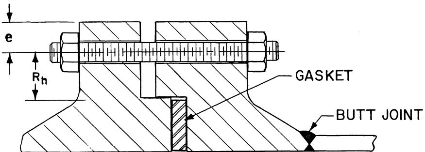
Fig. 3.3.1. Male and female joint (semi-confined).
