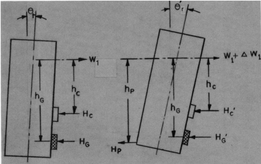
Fig. 3.14.1. Deflection of one of pair of identical flanges.
