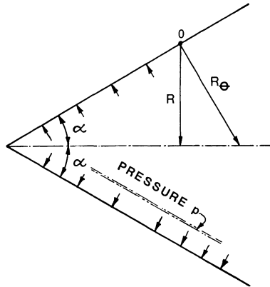
Fig. 13.4.1. Conical shell under internal pressure.
